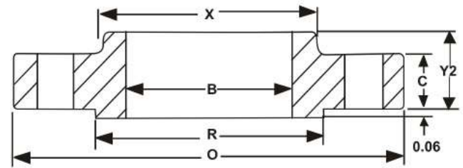
Slip On
