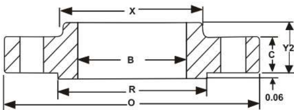
Slip On
