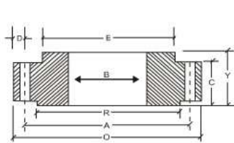
SLIP-ON FLANGE
