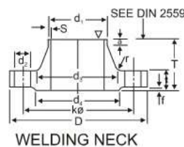
WELDING NECK
