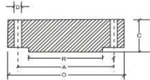
BLIND FLANGE
