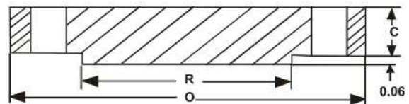
Blind
